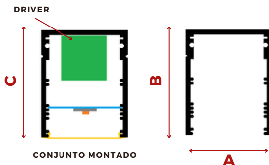
CHASSI / FITA LED
